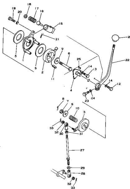
Fig. 121 FUEL CONTROL LEVER (適用機種: 1501~2200)
