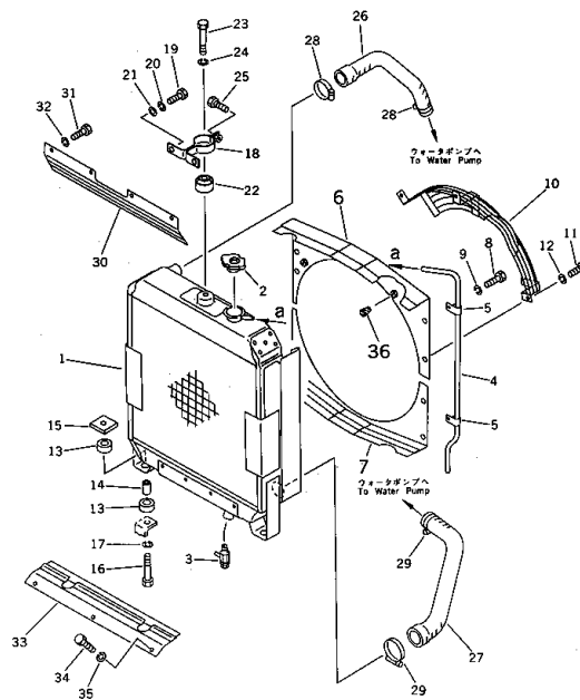
FIG.1203 RADIATOR AND PIPING (FOR 25A ALTERNATOR)
