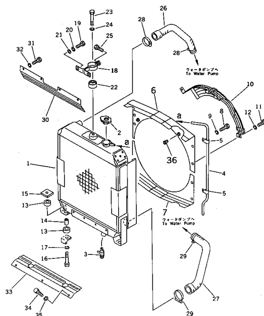
FIG.1203 25A 2501-UP 用 (25A 2501-UP 用) RADIATOR AND PIPING (FOR 25A ALTERNATOR)
