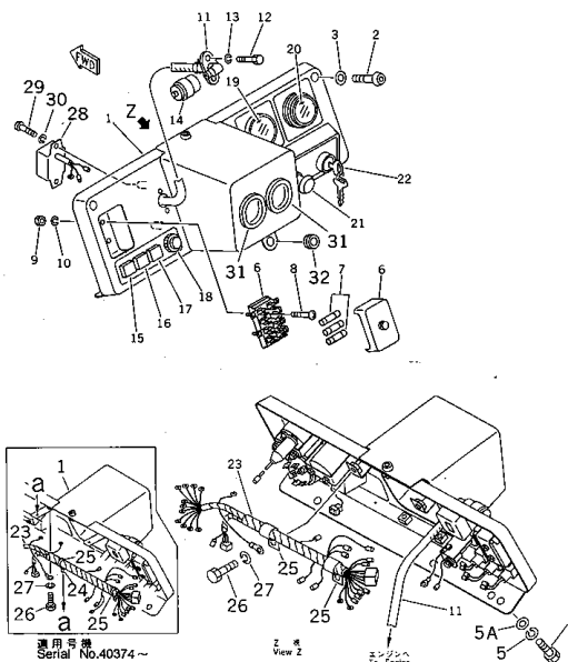
FIG.1411 030060 INSTRUMENT PANEL
