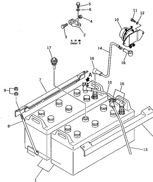
Fig. 4151 BATTERY (D31S Serial No.32001~32955) (D31Q Serial No.32001~32947)
