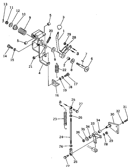
Fig. 4121 FUEL CONTROL LEVER (1/2)
