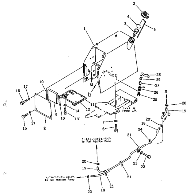
FIG.1307A FUEL TANK AND PIPING (TBG SPEC.)(#40238-)
