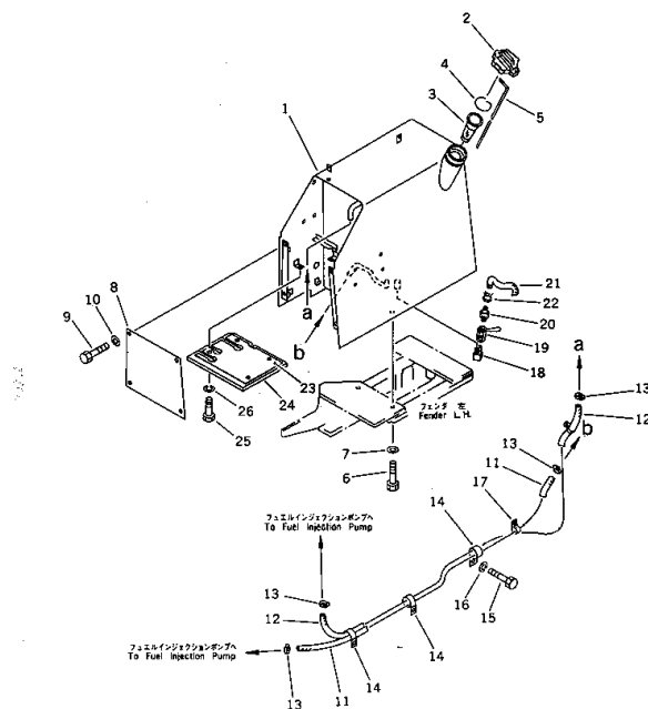
FIG.1307 FUEL TANK AND PIPING (TBG SPEC.) (#40001-40237)
