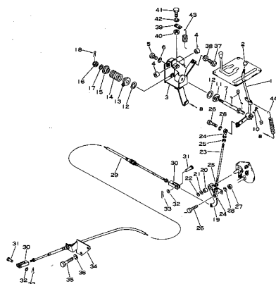
Fig. 3121 FUEL CONTROL LEVER
