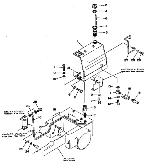
Fig. 3145 FUEL TANK AND PIPING- WITH ADDITIONAL FUEL FILTER (Except Japan) (Serial No. 25001~28000)
