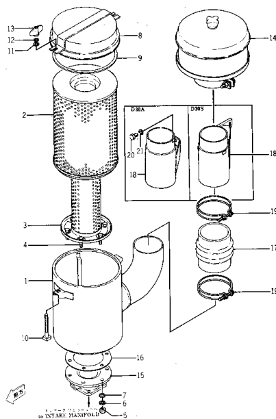
Fig. 102 AIR CLEANER AND CONNECTION (Serial No. 555~4999)
