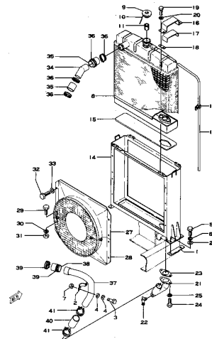
Fig. 121 RADIATOR AND MOUNTING (Serial No. 555-4999)
