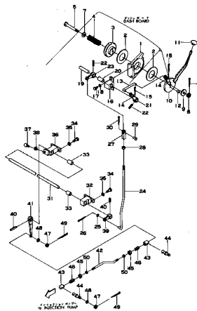
Fig. 1104 FUEL CONTROL LEVER
