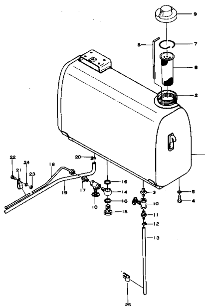
Fig. 1122 FUEL TANK AND PIPING
