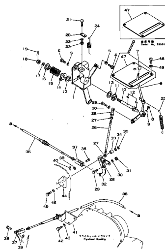
Fig. 3121 FUEL CONTROL LEVER
