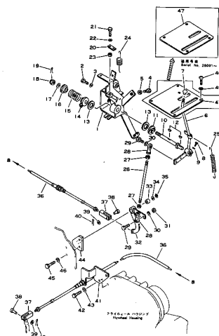
Fig. 3121 FUEL CONTROL LEVER
