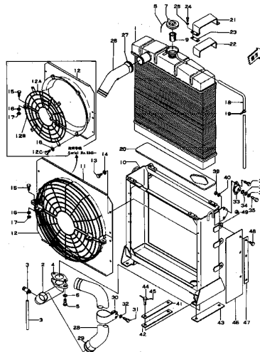
Fig. 1121 RADIATOR AND MOUNTING
