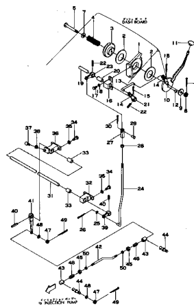
Fig. 1104 FUEL CONTROL LEVER
