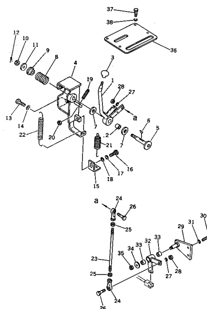
Fig. 121 FUEL CONTROL LEVER
