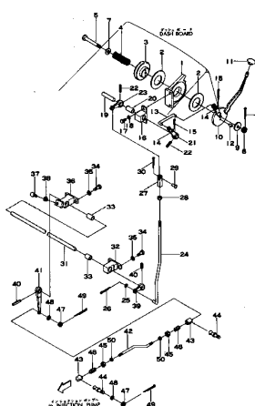
Fig. 1104 FUEL CONTROL LEVER
