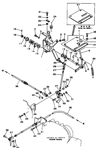
Fig. 3121 FUEL CONTROL LEVER
