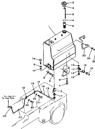
Fig. 3141 FUEL TANK AND PIPING 適用機種 (D30AF Serial No. 25633~28000) (D30PF Serial No. 25766~28000)
