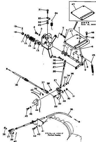
Fig. 3121 FUEL CONTROL LEVER
