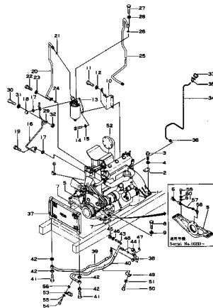
Fig. 1102 ENGINE RELATED PARTS (D30A, P Serial No. 5004--)
