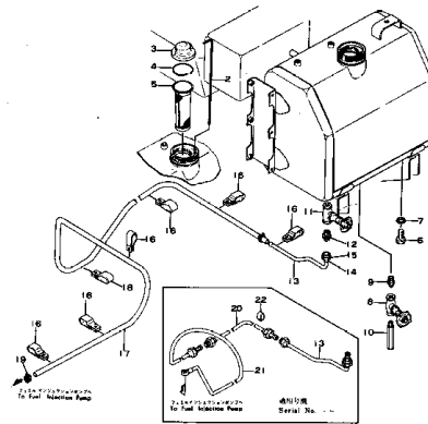
Fig. 1132 FUEL TANK AND PIPING (D21-3)
