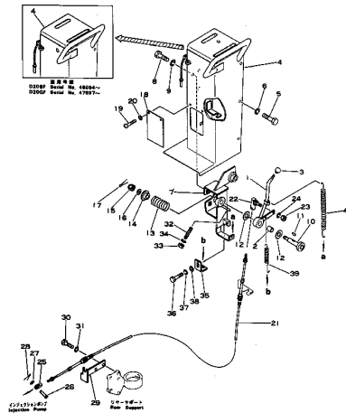
Fig. 2121 FUEL CONTROL LEVER
