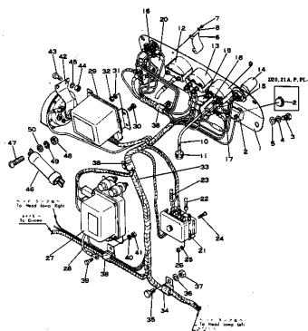
Fig. 1141 INSTRUMENT PANEL REGULATOR AND FUSE BOX
