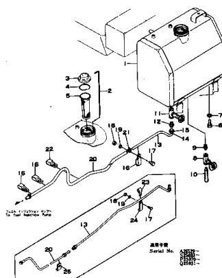
Fig. 1131 FUEL TANK AND PIPING (D20-3)
