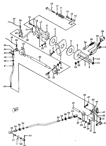
Fig. 103A FUEL CONTROL LEVER (Serial No. 2081~)
