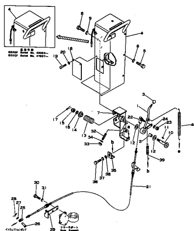
Fig. 2121 FUEL CONTROL LEVER
