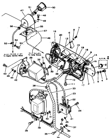
Fig. 1141 INSTRUMENT PANEL REGULATOR AND FUSE BOX
