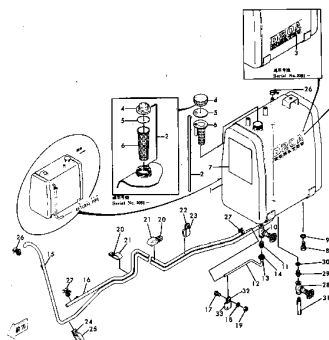
Fig. 127 FUEL TANK AND PIPING (適用車種: Serial No. 1005-)
