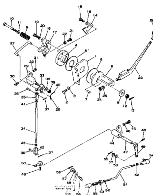
Fig. 1102 FUEL CONTROL LEVER
