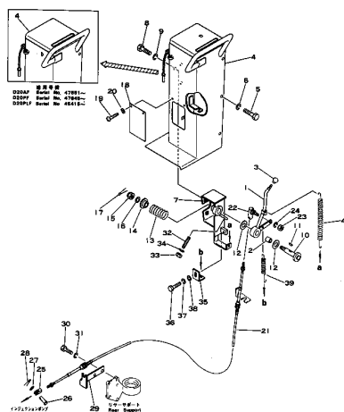
Fig. 3121 FUEL CONTROL LEVER
