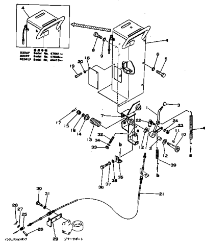
Fig. 3121 FUEL CONTROL LEVER
