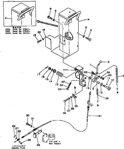
Fig. 3121 FUEL CONTROL LEVER
