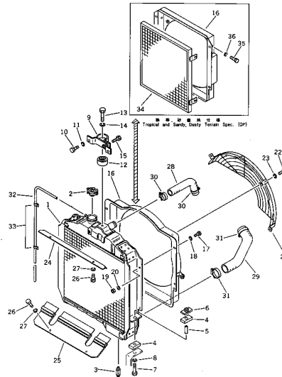
Fig. 3131A RADIATOR AND PIPING (D20A Serial No. 53687 ~ / (D20P Serial No. 53407 ~ ) (D20PL Serial No. 50626 ~ )
