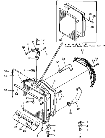
Fig. 3131 RADIATOR AND PIPING (D20A Serial No. 45001 ~ 53686 / (D20P Serial No. 45003 ~ 53406) (D20PL Serial No. 45001 ~ 50625)
