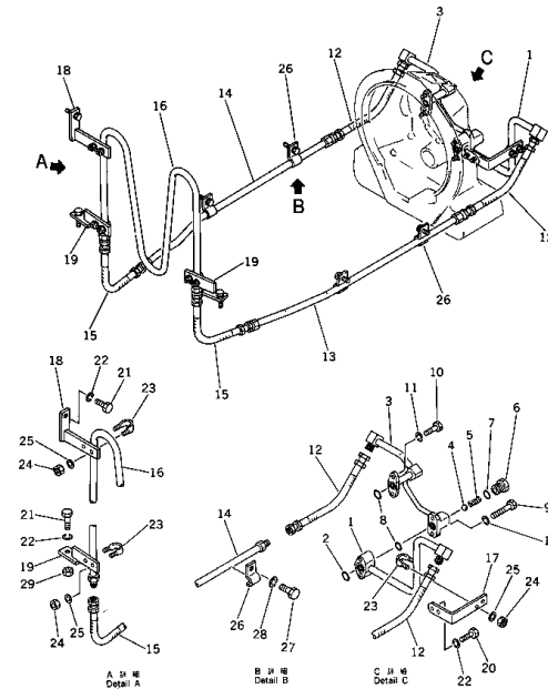
Fig. 3135 OIL COOLER AND PIPING
