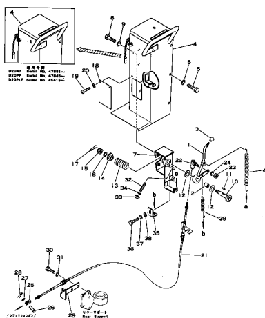
Fig. 3121 FUEL CONTROL LEVER
