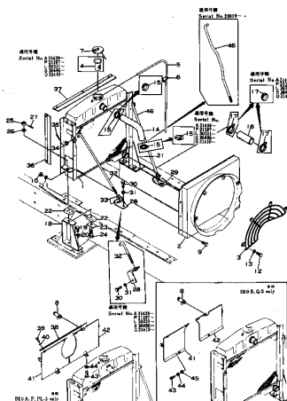
Fig. 1121 RADIATOR (D20-3)
