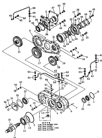
FIG.105 P.T.O. 9-9 87 POWER TAKE OFF
