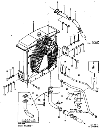
Fig. 1121A RADIATOR RELATED PARTS (Serial No. 2501~3344)
