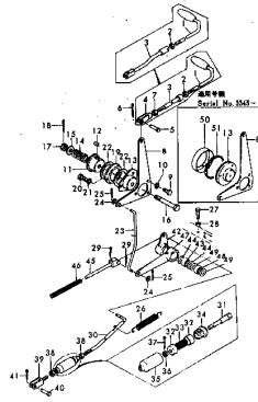
Fig. 1105 ACCELERATOR LEVER (Torqueflow Drive)
