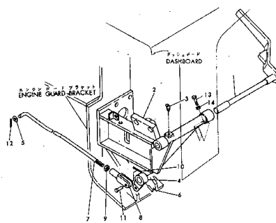
Fig. 1107 COMPRESSION RELEASE
