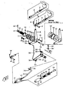
Fig. 1106 ACCELERATOR LEVER (Direct Drive)
