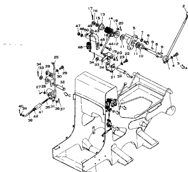
Fig. 111 FUEL CONTROL LEVER
