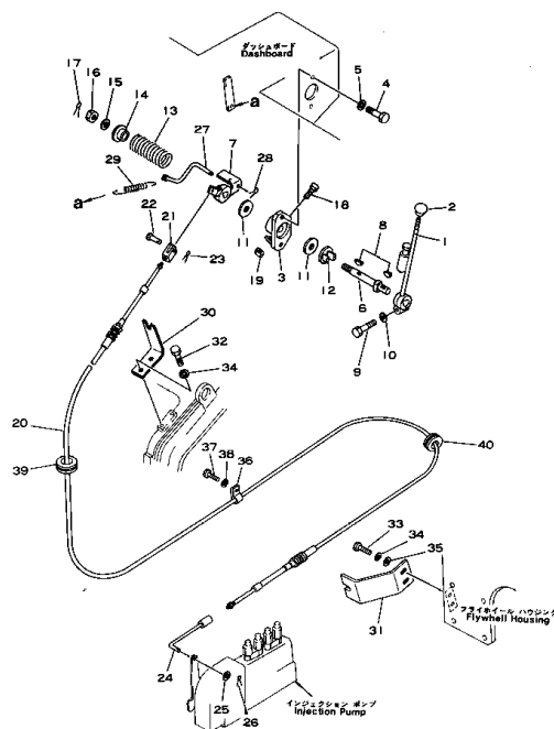
Fig. 121 FUEL CONTROL LEVER
