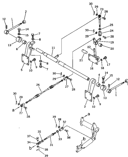
Fig. 123A FUEL CONTROL LEVER (2/2) (CD40C Serial No. 1179~)
