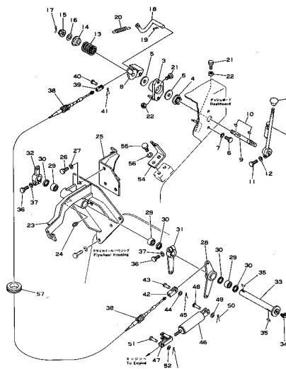
Fig. 122 FUEL CONTROL LEVER (1/2) (CD40C Serial No. 1001~)
