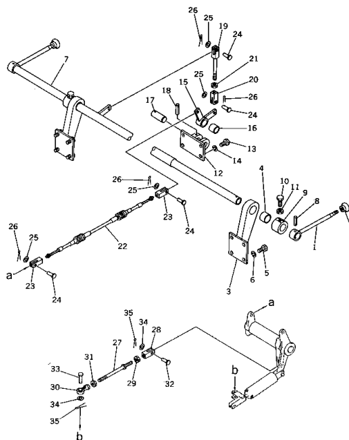
Fig. 123 FUEL CONTROL LEVER (2/2) (CD40C Serial No. 1001~1178)
