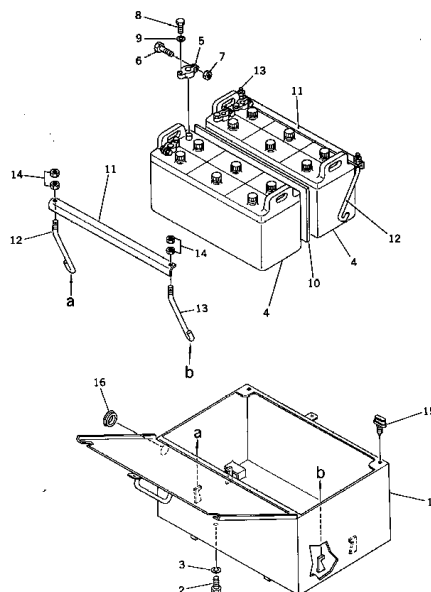
Fig. 151 BATTERY
