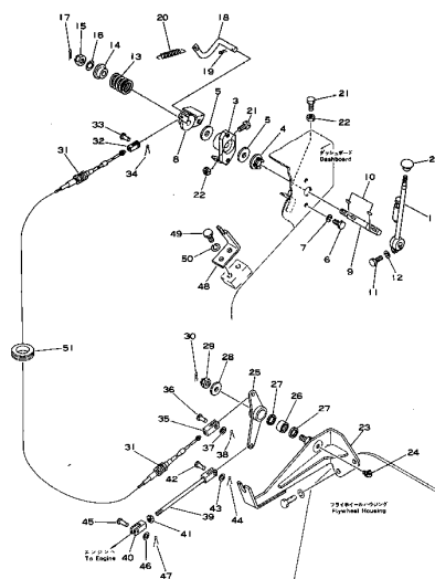
Fig. 121 FUEL CONTROL LEVER (CD40 Serial No. 1001~)
