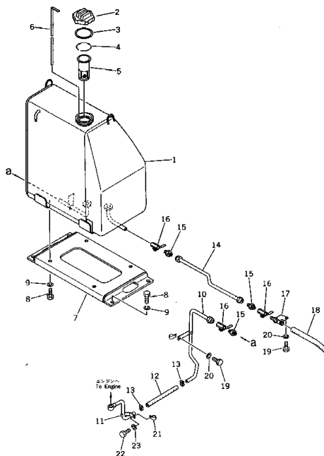
Fig. 141A FUEL TANK AND PIPING (CD40 Serial No. 1150~) (CD40C Serial No. 1150~)
