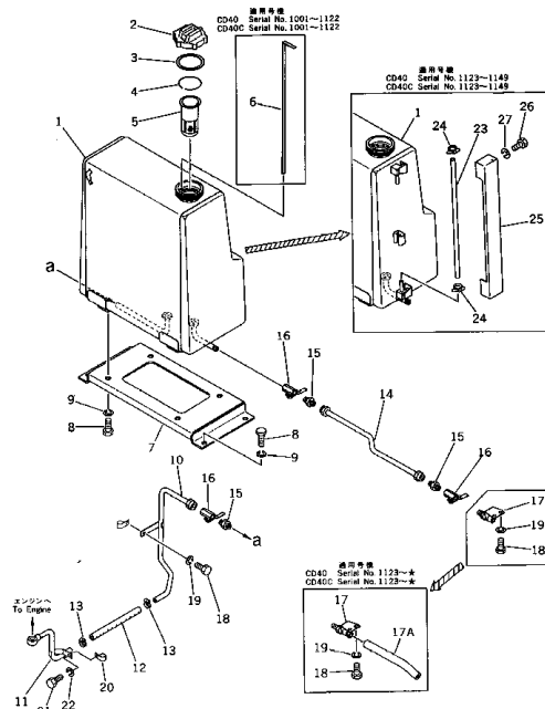
Fig. 141 FUEL TANK AND PIPING (CD40 Serial No. 1001~1149) (CD40C Serial No. 1001~1149)
