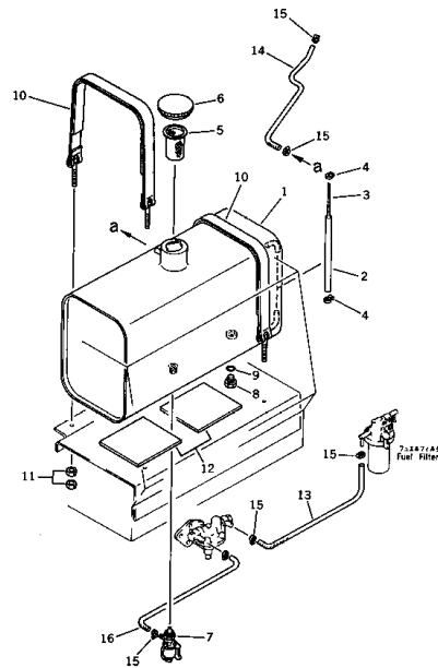
Fig. 141 FUEL TANK
