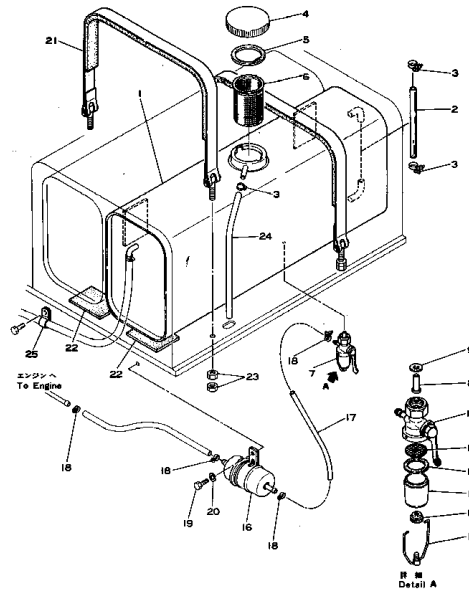
Fig. 142 FUEL TANK AND PIPING (CD25C)
