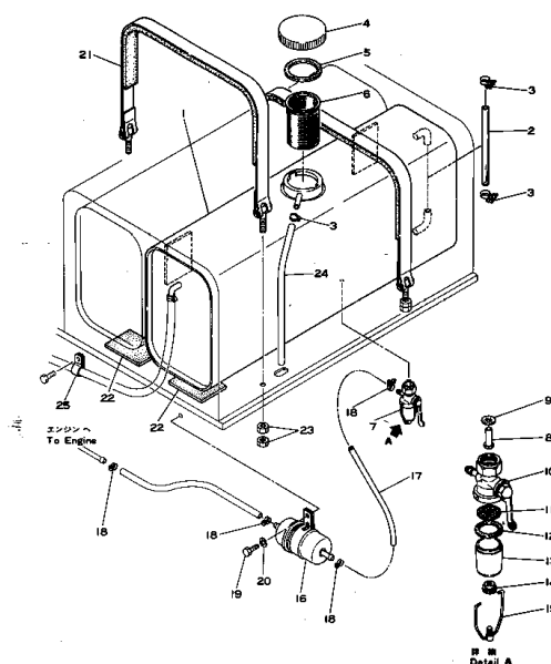
Fig. 142 FUEL TANK AND PIPING (CD25)
