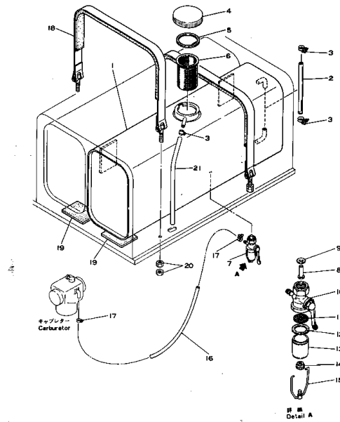
Fig. 141 FUEL TANK AND PIPING (CD20)
