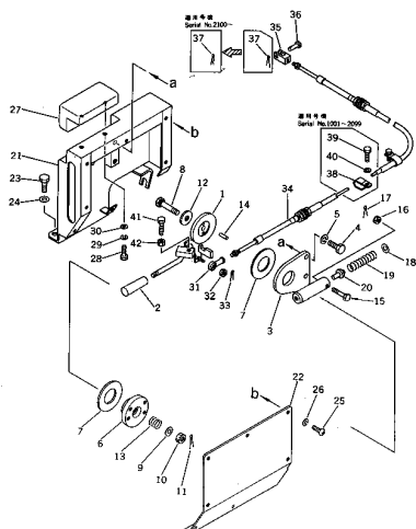
Fig. 121 FUEL CONTROL LEVER
