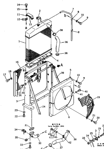
Fig. 131A RADIATOR AND COOLING (Serial No. 2001-)
