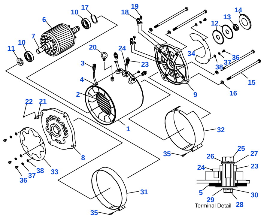
G-3 FIG. 17-0002 TRACTION MOTOR (UL EE) FB20/25/30/32SHE-6, FB20/25SHGE-6 - S/N 90001A~/93001~
