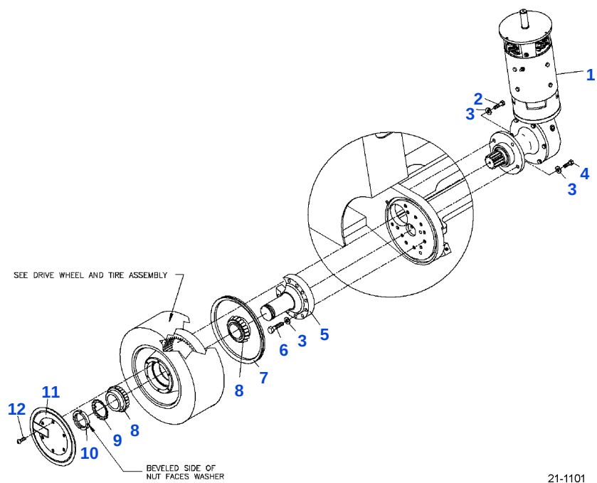
A-1 FIG. 21-1101 DRIVE TRAIN ASSEMBLY
