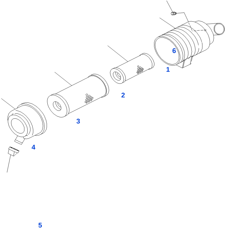
A-17 FIG. A4140-51A0 ENGINE - SAA4D95LE - AIR CLEANER - DETAIL ENGINE S/N 503377~ / TRUCK S/N 55001~
