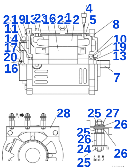
FIG. G4110-51A0 TRACTION MOTOR (INNER PARTS)
