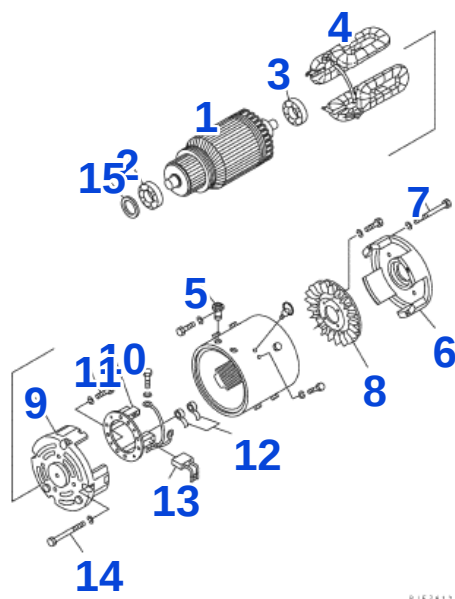
FIG. G4130-51A0 PUMP MOTOR (INNER PARTS)
