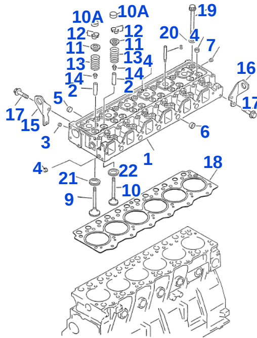
Fig. 102 CYLINDER HEAD (W)
