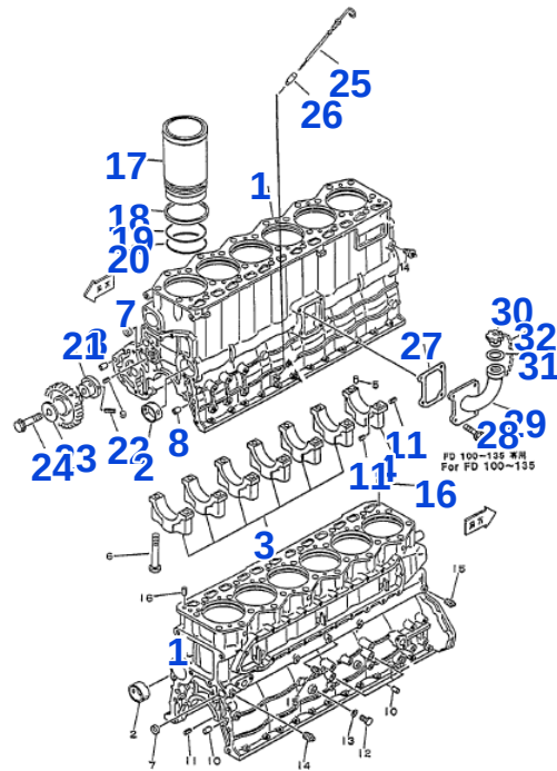
FIG. 201 CYLINDER BLOCK
