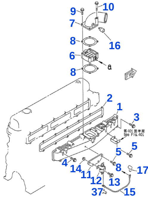
FIG. 111 AIR INTAKE MANIFOLD AND CONNECTION
