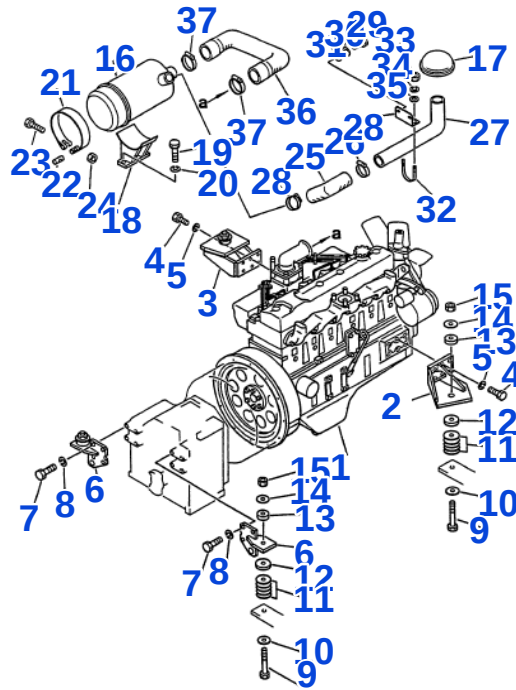
FIG.1001 ENGINE MOUNTING PARTS (FOR 6D95L)
