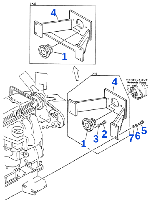
FIG.1065 PUMP DRIVE SYSTEM (FOR P40)
