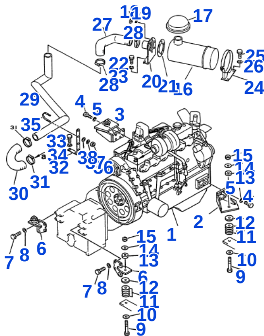
FIG.1021 ENGINE MOUNTING PARTS (FOR S6D95L)
