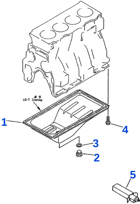
Fig. 211 OIL PAN
