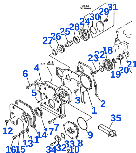
Fig. 205 FRONT COVER AND GEAR
