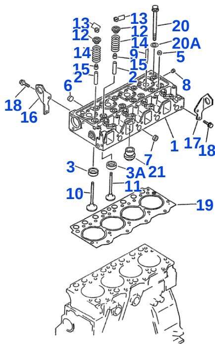
Fig. 101 CYLINDER HEAD
