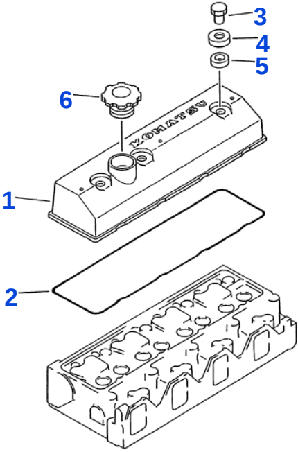
Fig. 105 CYLINDER HEAD COVER
