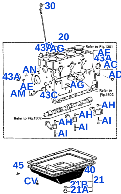
FIG.1105 CYLINDER BLOCK
