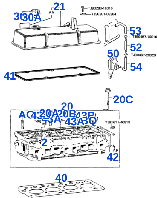
FIG.1104 CYLINDER HEAD &amp; VENTILATION HOSE
